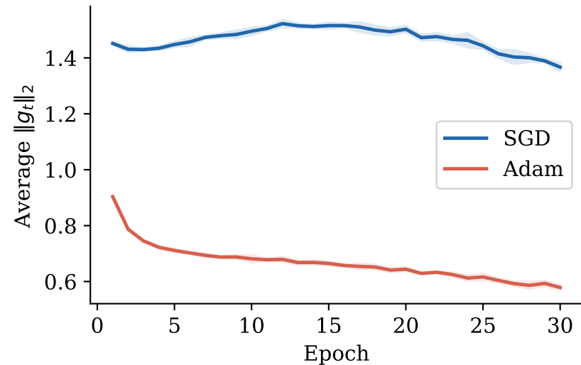
(a) MLP
