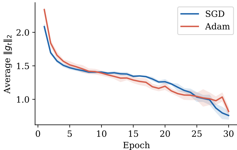
(b) SmallCNN
